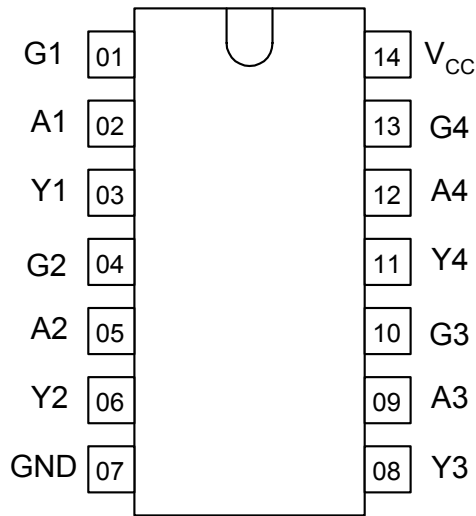
Pinout
