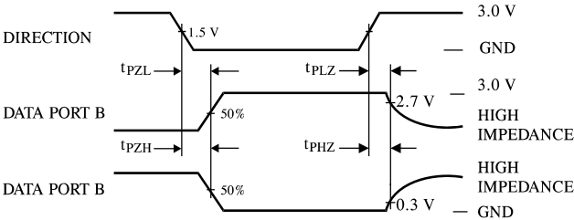
Figure 6. Switching Waveforms
