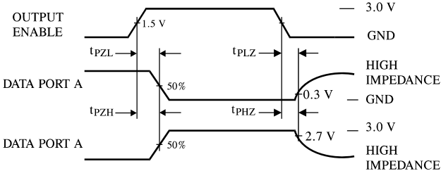
Figure 5. Switching Waveforms
