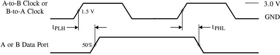
Figure 1. Switching Waveforms
